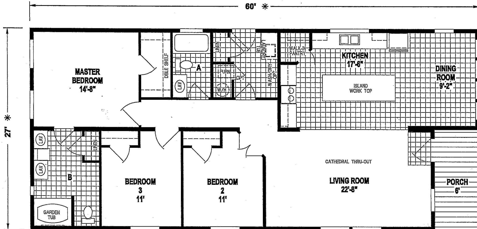
OPT WINDOW 1265CT/6028 (1,620 SQ. FT.) 3BEDROOM - 2BATHS - CATHEDRAL THRU-OUT
